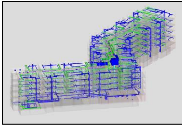
HVAC BIM MODELING
